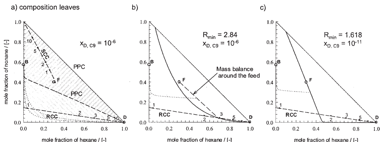
Figure 5. Minimum reflux case study for a mixture of hexane (1)–heptane (3)–nonane (2).
