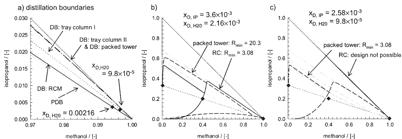
Figure 8. (a) Distillation boundaries close to pure methanol for four different MT models: RC (equal diffusivity model), tray column I ( C_1 = 1.1 , C_2 = 0.5 ), tray column II ( C_1 = 0.5 , C_2 = 1 ), packed tower ( C_1 = 0.6 , C_2 = 0.6667 ) (for all models, \mathcal{D}_{ref} = 5 \times 10^{-5} \text{ m}^2/\text{s} ); (b–c) composition profiles at minimum reflux for the packed tower and the equal diffusivity model. Light gray lines refer to the RRC and the pinch-point curves in Figure 6.
